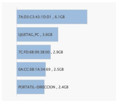
Client Trend
