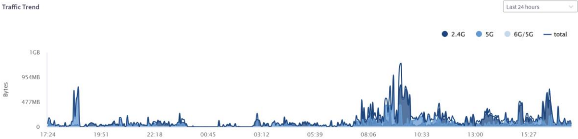
Traffic Trend
