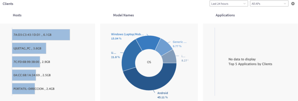
Clients
