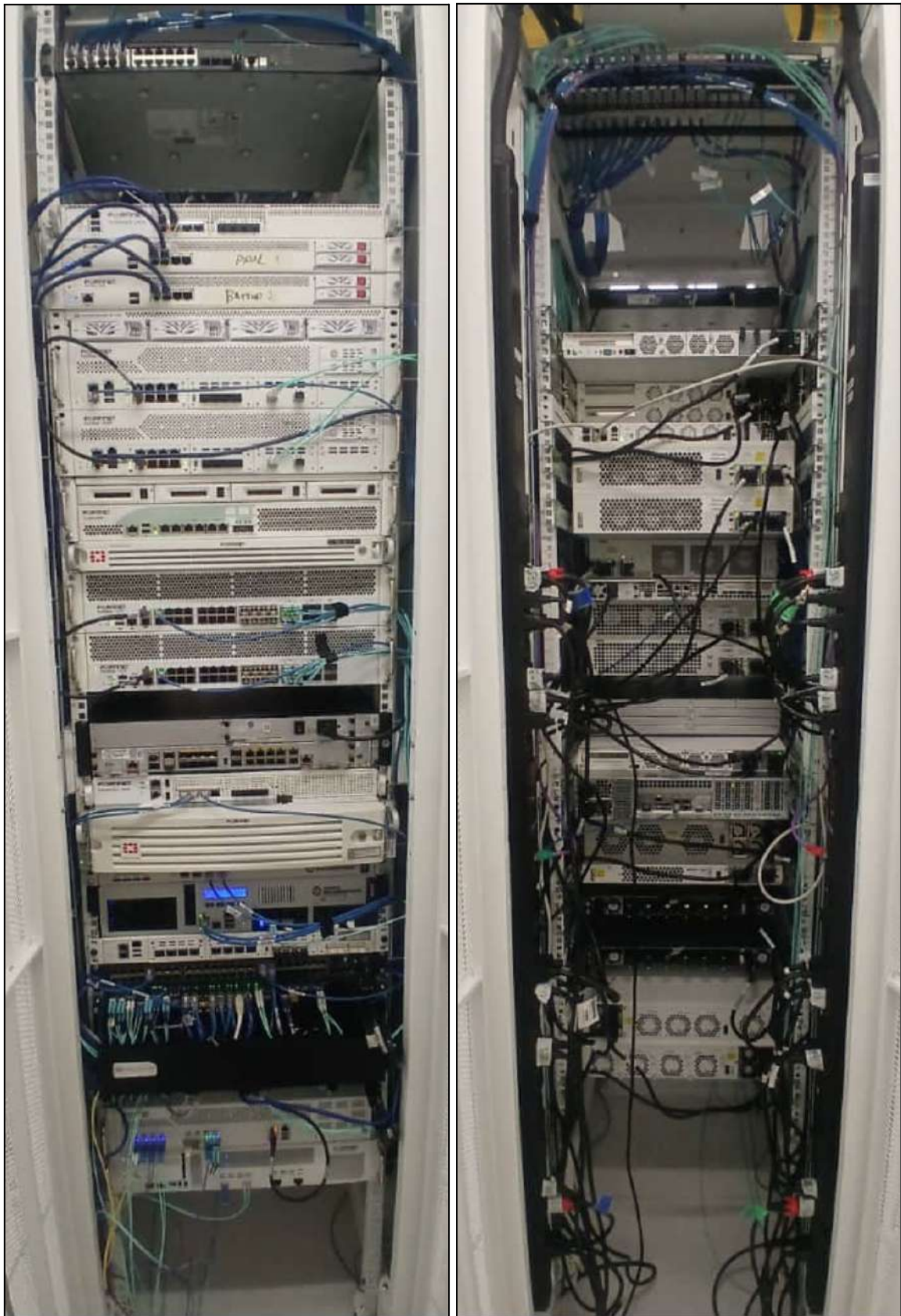
Figura 10 - Back & Front Rack 1H.10
