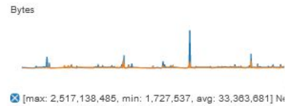
Network-ServidorPROXY-prod
