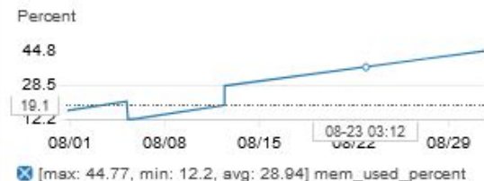
Memory-APIGWExterno-prod
