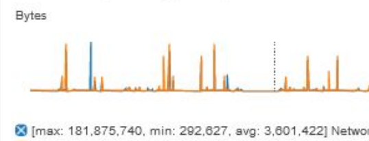
Network-CapadeNegocio2-prod
