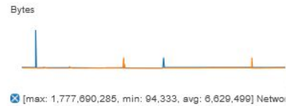
Network-ETL-prod
