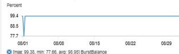
RDS BurstBalance-sqlserver
