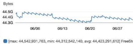
RDS FreeableMemory-sqlserver
