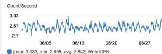
RDS WriteIOPS-postgres
