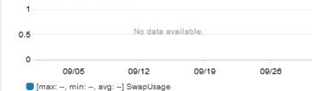
RDS SwapUsage-sqlserver
