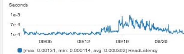
RDS ReadLatency-sqlserver
