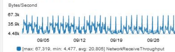
RDS NetworkReceiveThroughput-sqlserver
