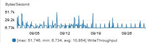
RDS WriteThroughput-sqlserver
