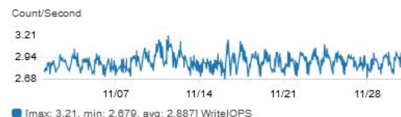
RDS WriteIOPS-postgres
