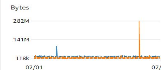
Network-ETL-prod
