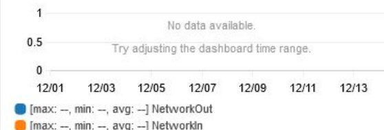
Network-ServidorPROXY2-prod
