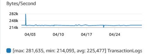
RDS TransactionLogsGeneration-postgres
